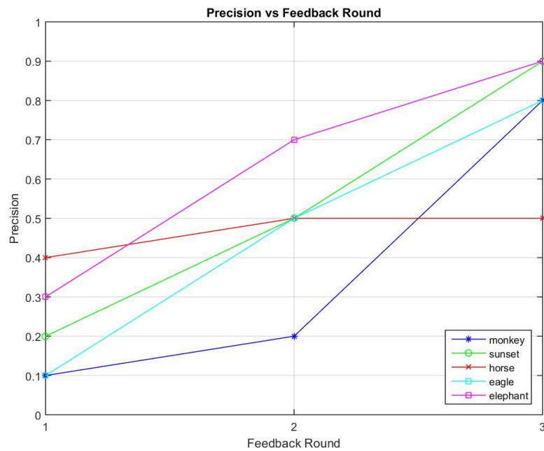
Fig 1: Precision Vs Feedback Round
